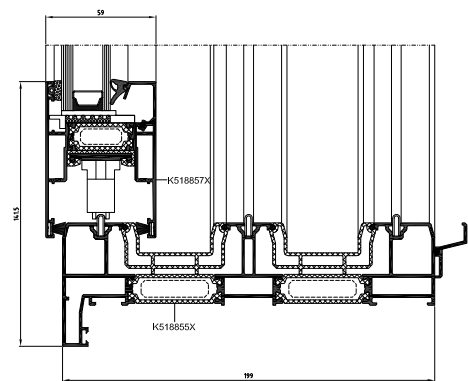
cross section of the bottom of the door with a triple-track renovation frame
