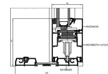
cross section of the bottom of a door with a low threshold
