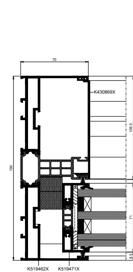
cross section of the side of the door
