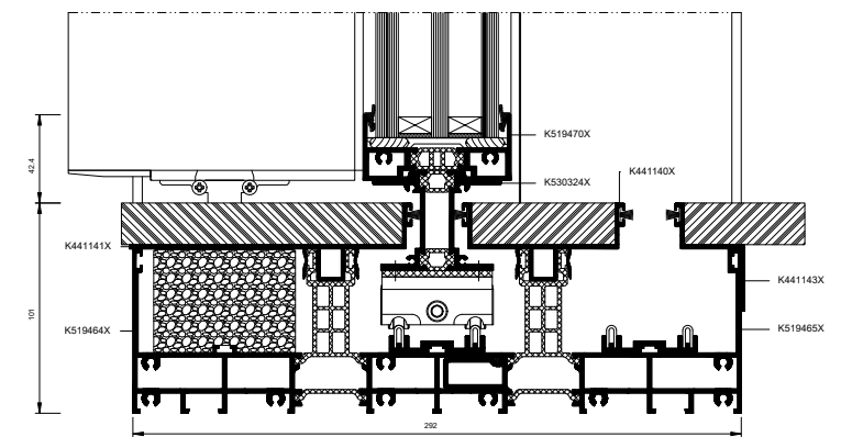
Door, bottom cross-section
