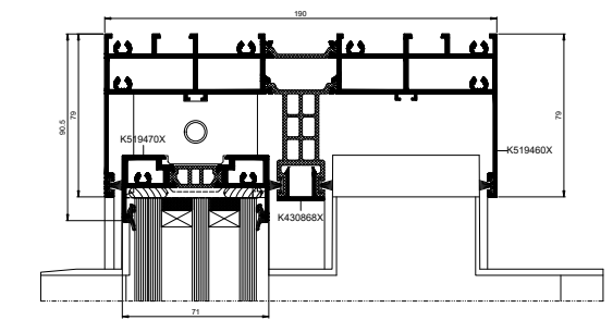
Door, top cross section
