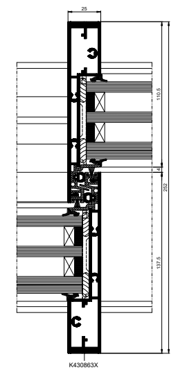
Door leaves connection, cross-section
