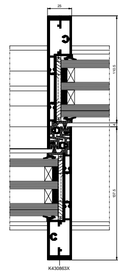
cross section of the door-leaf intersection point
