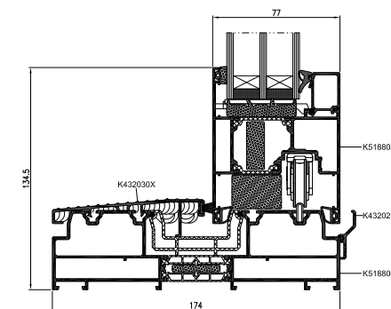
cross section of the door threshold
