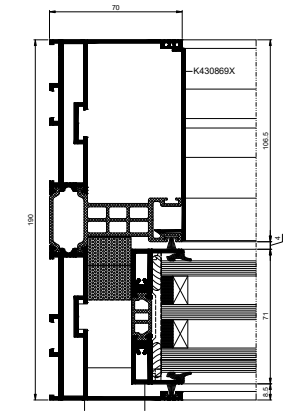
Door, side cross-section
