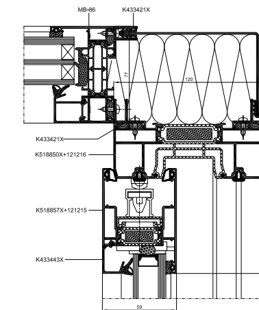
cross section through the 90° angle joint of the MB-59HS door with fixed window
