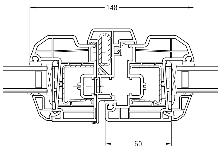
Small Dummy Mullion BriD, 550080 with Sash A 60 ED70, 550051
