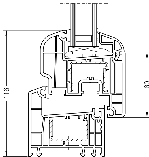
Frame 64 ED70, 550003 with Sash 60 round ED70, 550460
