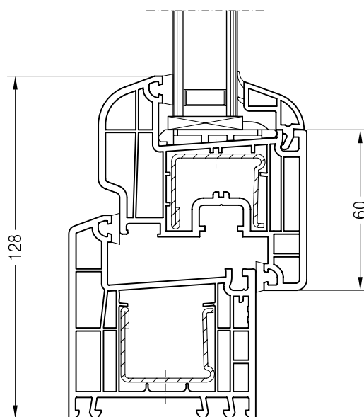
Frame 76-2 ED70, 550761 with Sash 60 round ED70, 550460
