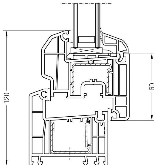
Frame 68 ED70, 550713 with Sash A 60 ED70, 550051
