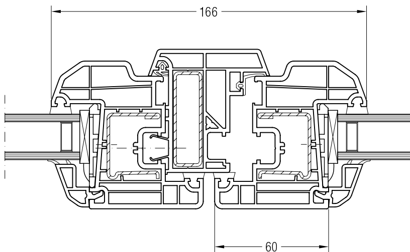
Dummy Mullion TD70, 550770 with Sash A 60 ED70, 550051
