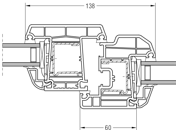
Mullion 86 ED70, 550813 with Sash A 60 ED70, 550051
