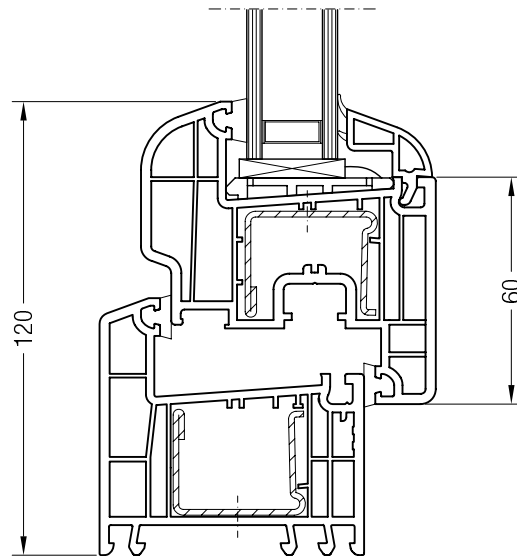
Frame 68 ED70, 550713 with Sash 60 round ED70, 550460
