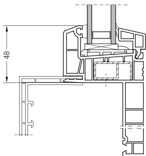
Precast Concrete Construction-Frame 37 or 60 ED70, 550999 or 550990
