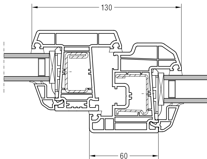
Mullion 78 ED70, 550613 with Sash A 60 ED70, 550051
