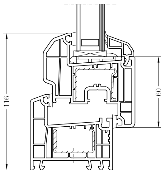
Frame 64 ED70, 550003 with Sash A 60 ED70, 550051
