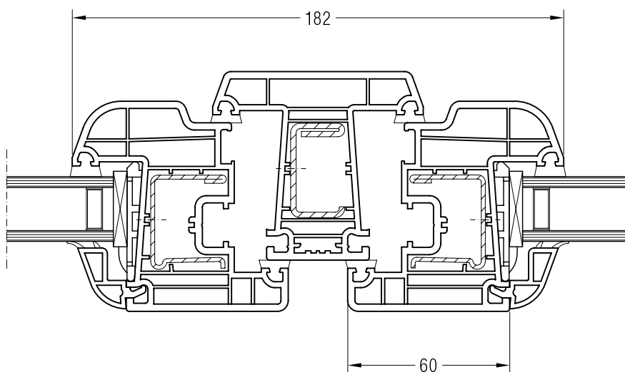
Mullion 78 ED70, 550613 with Sash 60 round ED70, 550460
