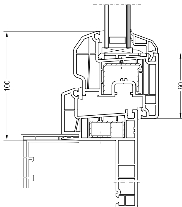
Precast Concrete Construction-Frame 37 or 60 ED70, 550990 or 550999,
