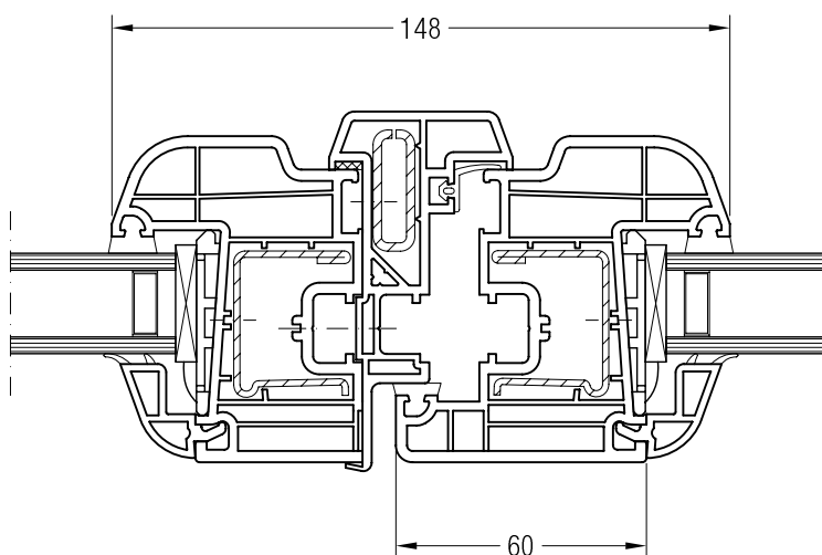
Small Dummy Mullion BriD, 550080 with Sash 60 round ED70, 550460
