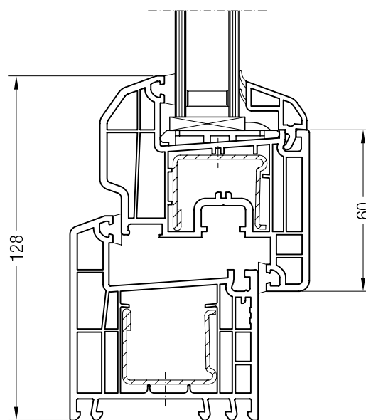
Frame 76-2 ED70, 550761 with Sash A 60 ED70, 550051
