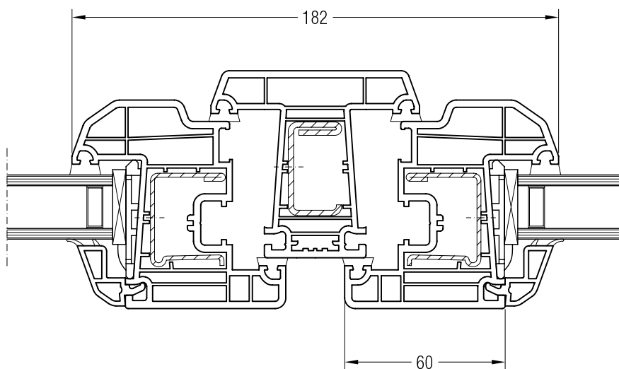
Mullion 78 ED70, 550613 with Sash A 60 ED70, 550051
