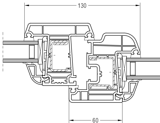
Mullion 78 ED70, 550613 with Sash 60 round ED70, 550460
