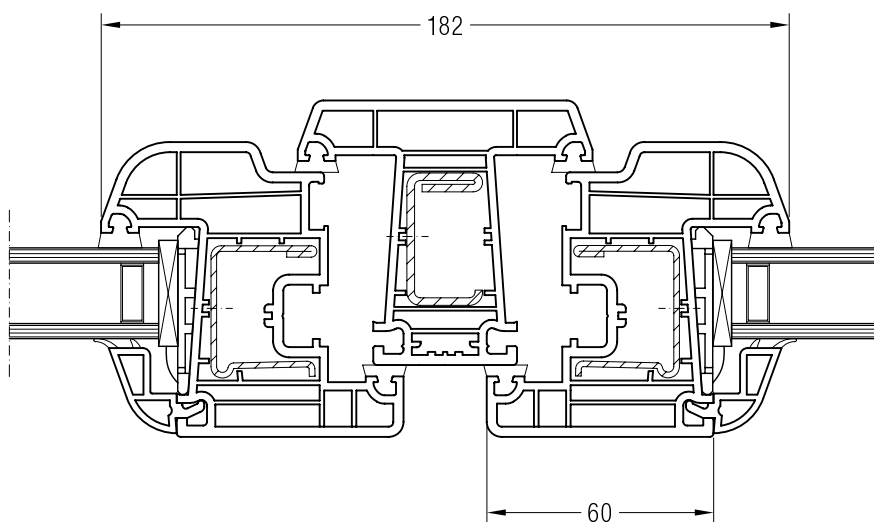
Mullion 86 ED70, 550813 with Sash 60 round ED70, 550460
