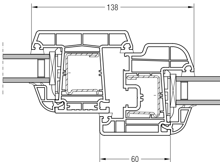
Mullion 86 ED70, 550813 with Sash 60 round ED70, 550460
