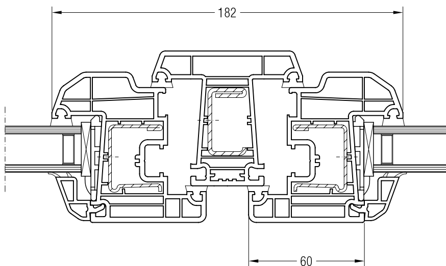
Mullion 86 ED70, 550813 with Sash A 60 ED70, 550051
